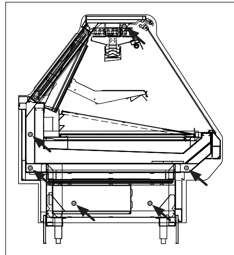
Fig. 3 Bolt locations
