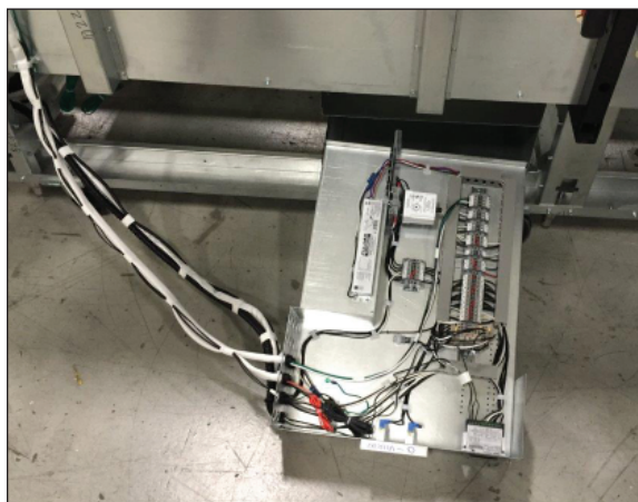
Fig. 8 Power supply box
