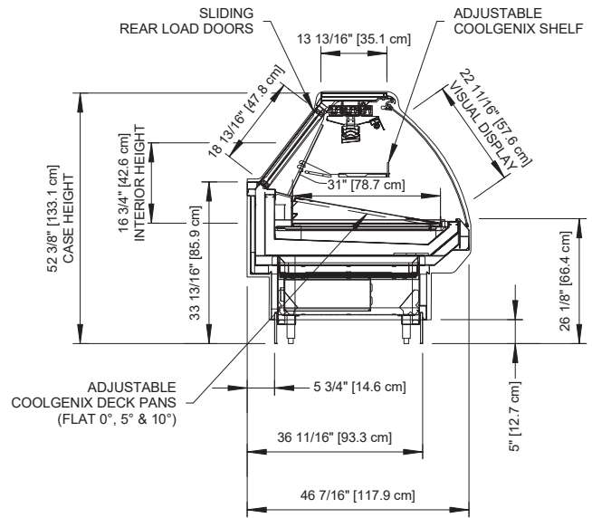
CURVED GLASS
