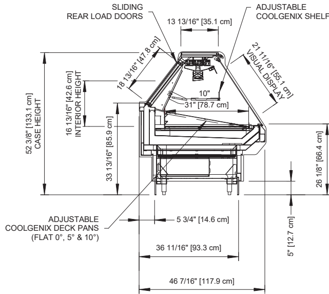
FLAT GLASS
